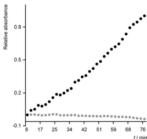
Figure 4. Progress curve for GOx polymersomes with surface-conjugated HRP. Two types of polymersomes are incubated with glucose and ABTS, and the appearance of ABTS •+ is measured as a function of time. After a short initial incubation period, polymersomes that only contain GOx do not show any increase in absorbance (grey dots). Polymersomes in which both enzymes are present do show an increasing concentration of ABTS •+ (black dots).
