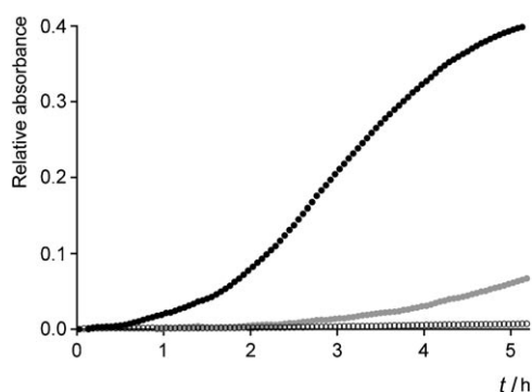
Figure 5. Progress curve for the three-enzyme cascade reaction (see Figure 2). The black dotted line shows the increasing concentration of the final product of the cascade, ABTS •+ . After filtration of the solution to remove polymersomes, no further enzymatic activity could be detected (open dots). The system that lacked CalB still showed activity due to chemical hydrolysis of 4 (grey dots).
