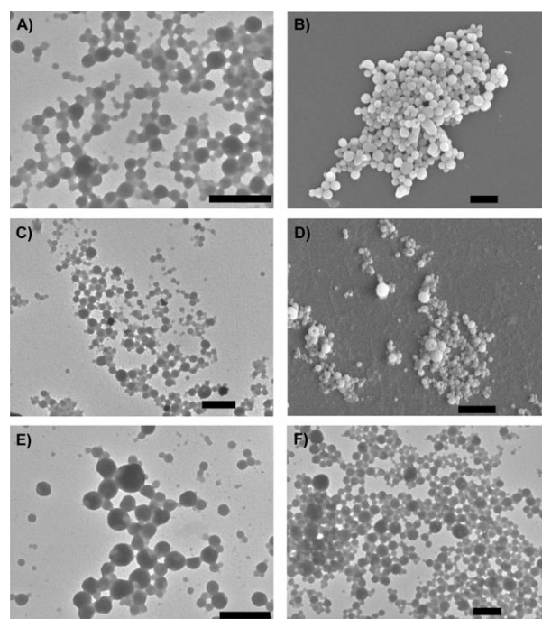
Figure 3. Electron micrographs of the biohybrid polymersomes. All micrographs shown are of PS-PIAT vesicles containing an admixed 10 wt % of 1 . The scale bar represents 500 nm. Their enzymatic content is as follows: A) GOx in the lumen (TEM); B) GOx in the lumen, HRP on the surface (SEM); C) GOx in the lumen, CalB in the membrane, HRP on the surface (TEM); D) GOx in the lumen, CalB in the membrane, HRP on the surface (SEM); E) 3-labelled GOx in the lumen (TEM); F) 3-labelled CalB in the membrane.
