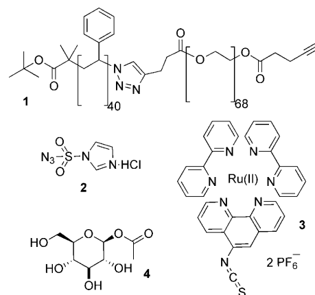
Scheme 1. Structures of block copolymer “anchor” 1 , diazo transfer reagent 2 , Ru-labelling compound 3 and glucose acetate 4 .
